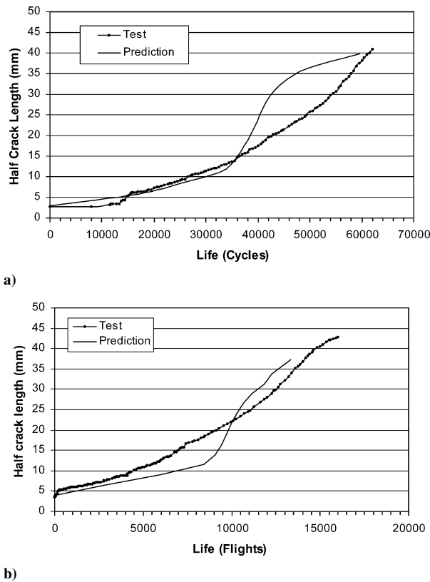
Fig. 5 Fatigue crack growth life in stringer web of the two-stringer tension panel; prediction vs test: a) constant-amplitude loading ( \sigma_{\max} = 88 MPa, R = 0.1 ); and b) aircraft service load spectrum ( \sigma_{\max} = 138 MPa).
