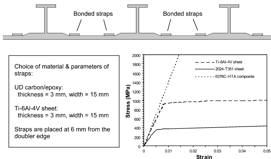
Fig. 11a Schematic of strap design considerations: geometry and material.
