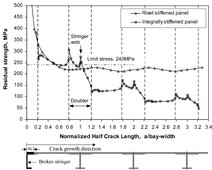
Fig. 10 Skin fracture curves for both integral and riveted panels.
