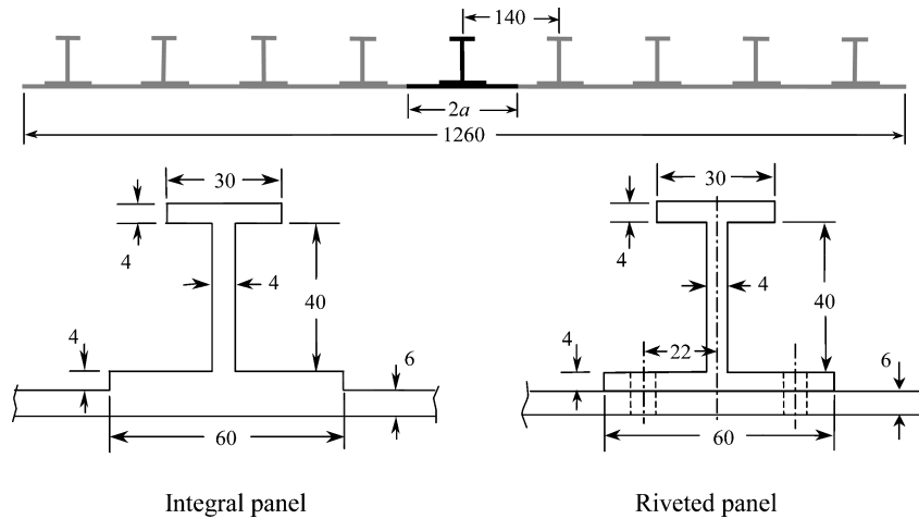
Fig. 3 Nine-stringer panels for generic analysis ( A_{st}/bt = 0.62 ). This geometry was used for three cases: riveted, integrally machined, and welded integral panels, for comparison in damage tolerance and fail-safety performance.
